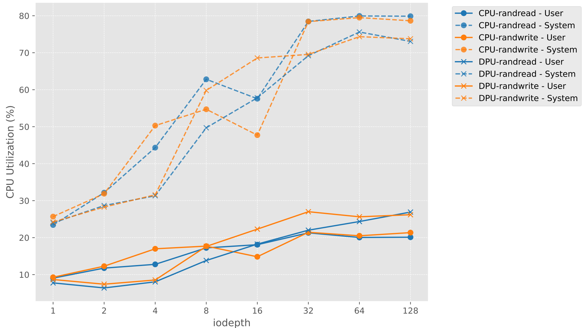
CPU Utilization vs iodepth (Random)
